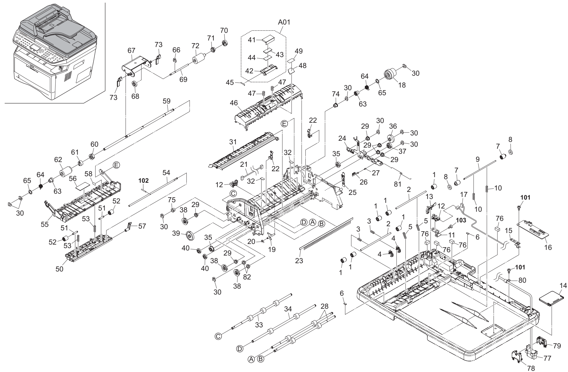
FIG. 14 Document Processor 1
