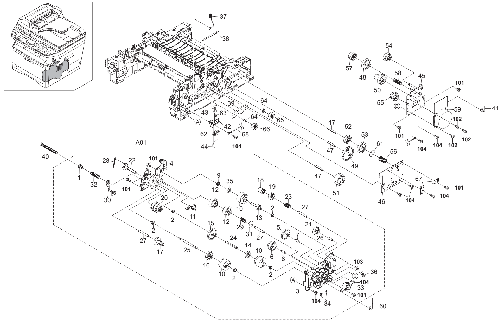
FIG. 10 Drive Section
