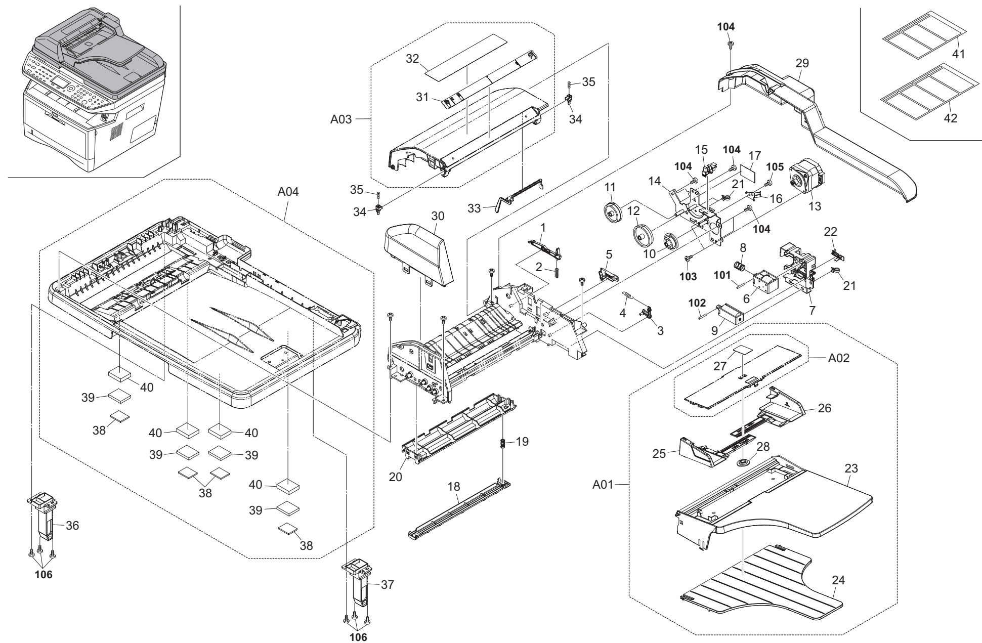
FIG. 15 Document Processor 2
