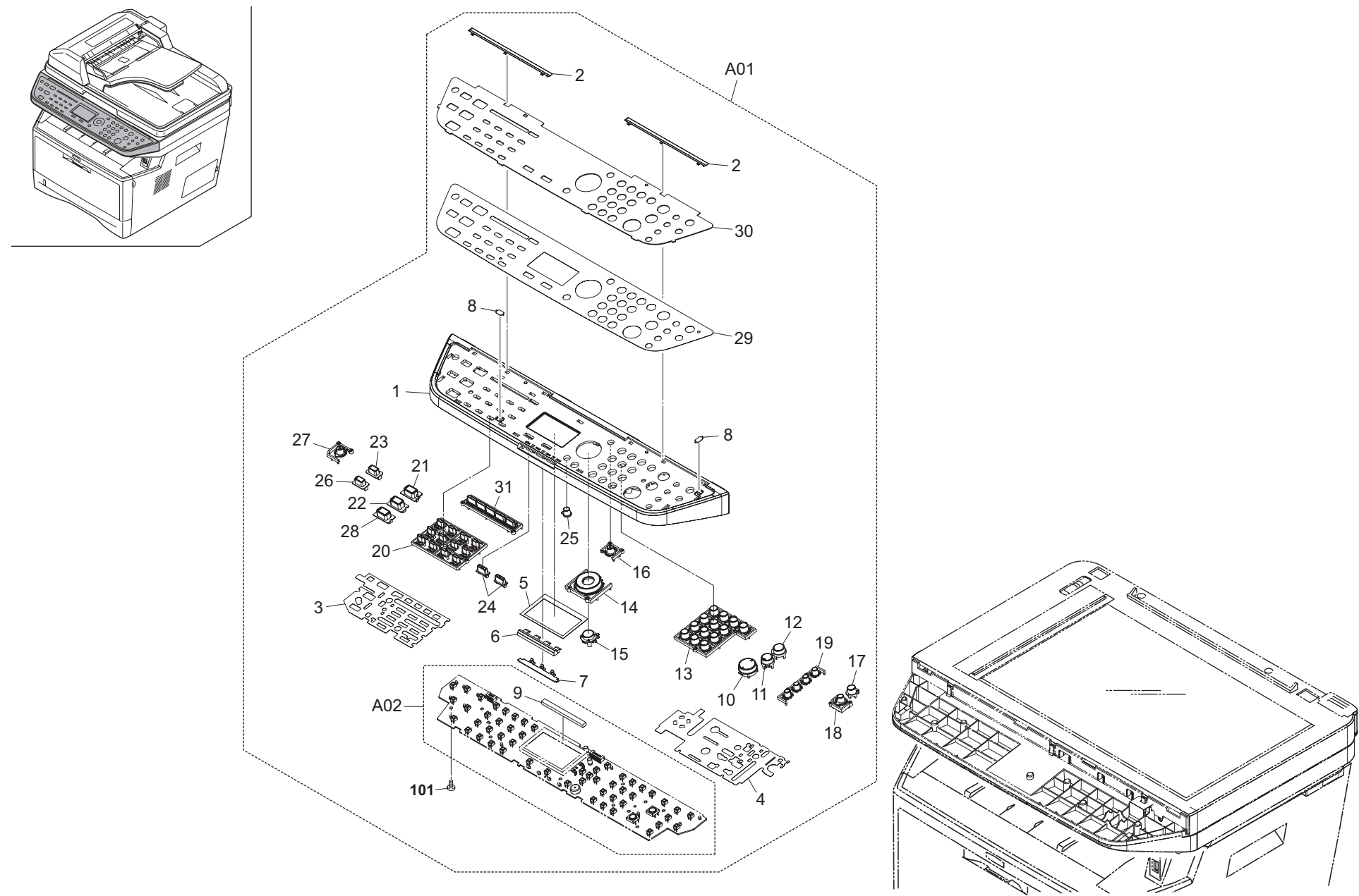
FIG. 13 Operation Section
