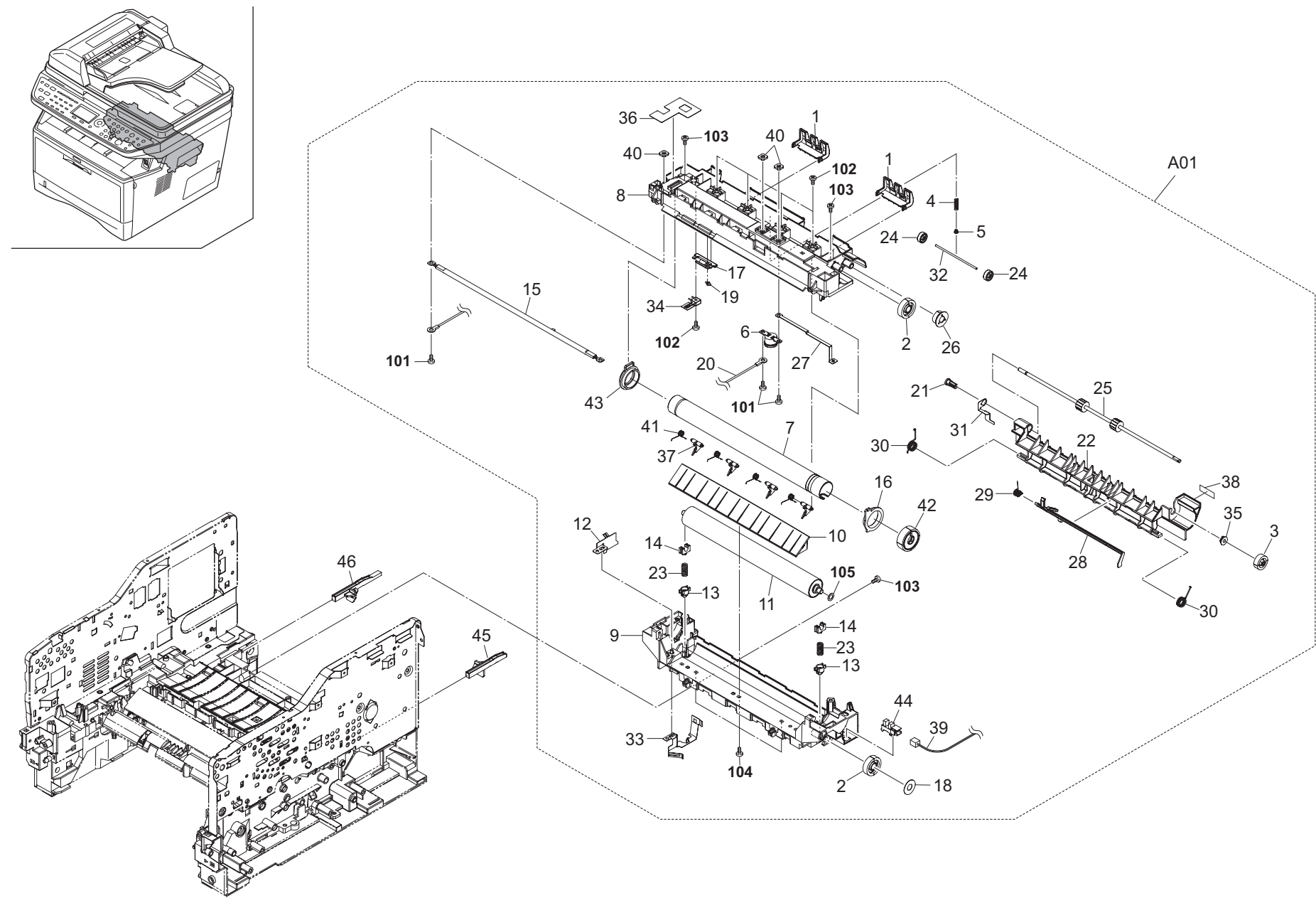
FIG. 9 Fuser Section
