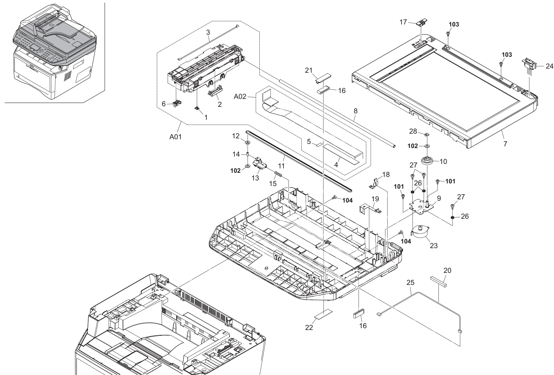
FIG. 6 Scanner Section
