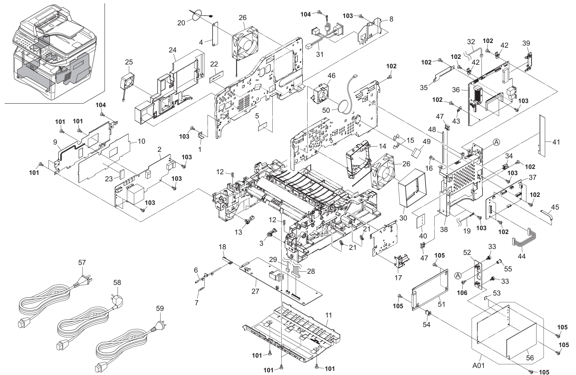
FIG. 12 Electrical Components
